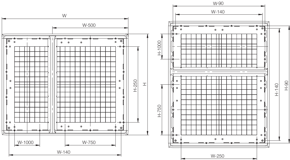
Front view W=1250 (without doors)
